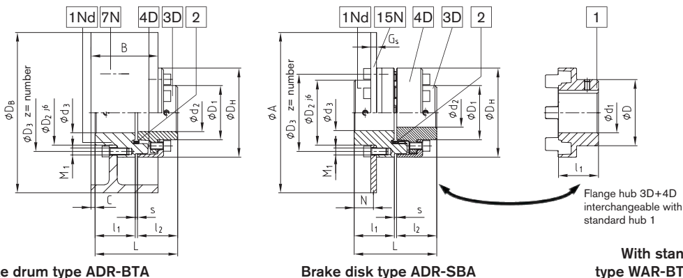
Brake drum type ADR-BTA
